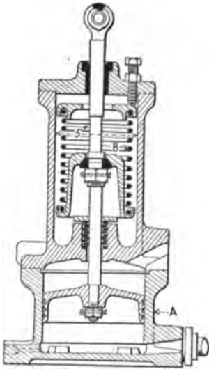
FIG. 104.—Piston controlled by multiplicator.
